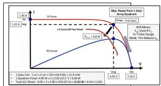
Figure 10: AO-7 Solar Cell I-V Characteristic (for One Solar Array Quadrant)
