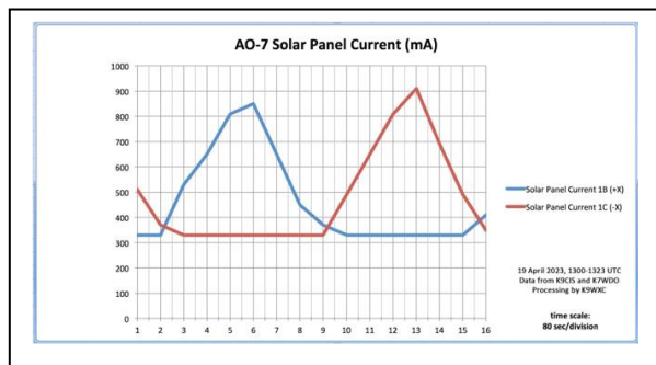
Figure 19: M.C. Telemetry of +X and -Y Solar Panel Current
