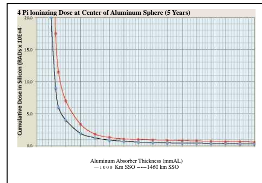
Figure 12: Dose Depth Curve; 5 Years for 1460 km SSO
