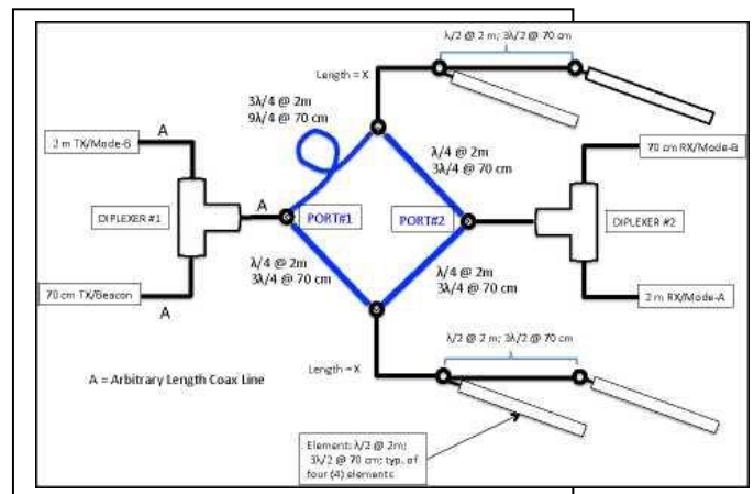
Figure 9: The AO-7 VHF/UHF Antenna Combiner Concept Using a 90 Coax Hybrid
