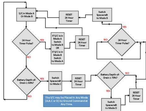
Figure 7: ECL Logic Flow Diagram
