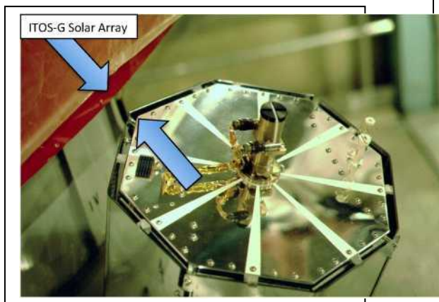
Figure 13: AO-7 and ITOS-G Proximity on Delta-
